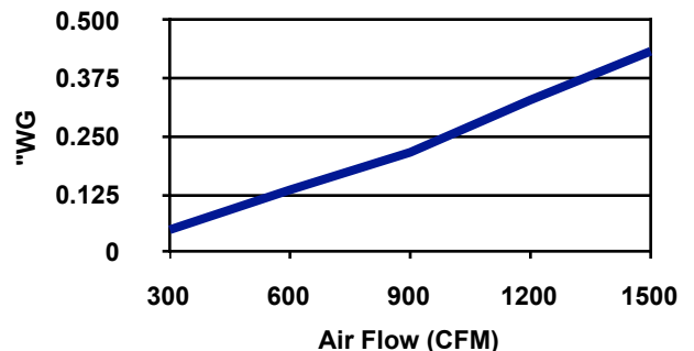
Air Flow vs. Resistance (Clean Filter)
